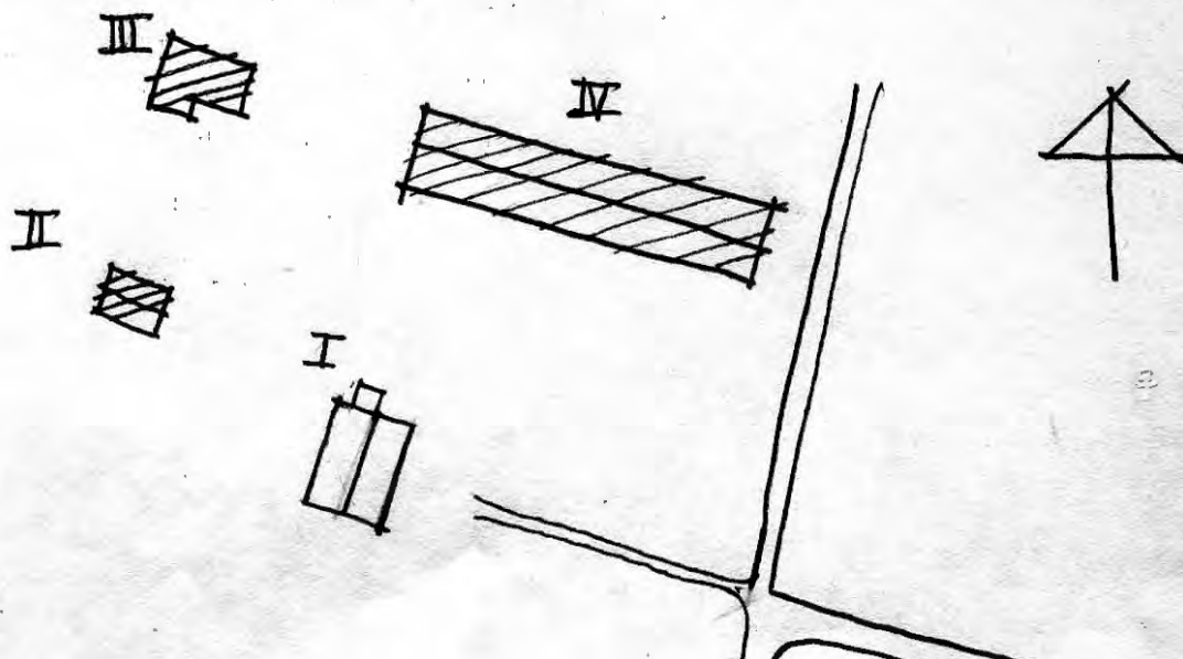
Situationsplan
