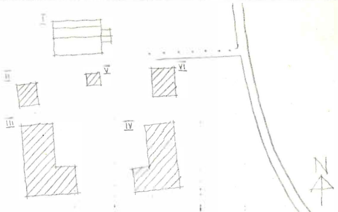
Situationsplan
